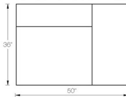
Chair & Half C (34" Seat with Table)
